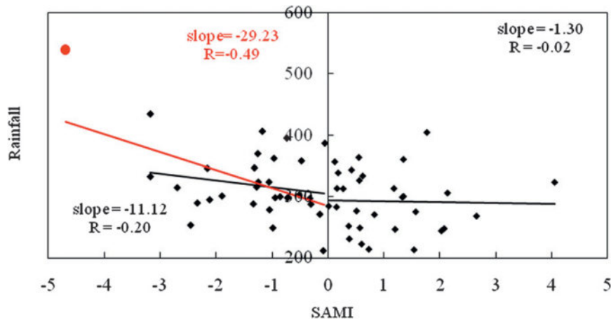
FIG. 2. Scatterplot of the winter SAMI against SWR. Black lines are linear fits for data of negative and positive SAM phases, for which the correlation and regression coefficients are shown. The red outlier (minimum SAM in 1964) is not included in the linear fit shown by the black line, but it is included in the linear fit for the negative SAM phase (red line).
