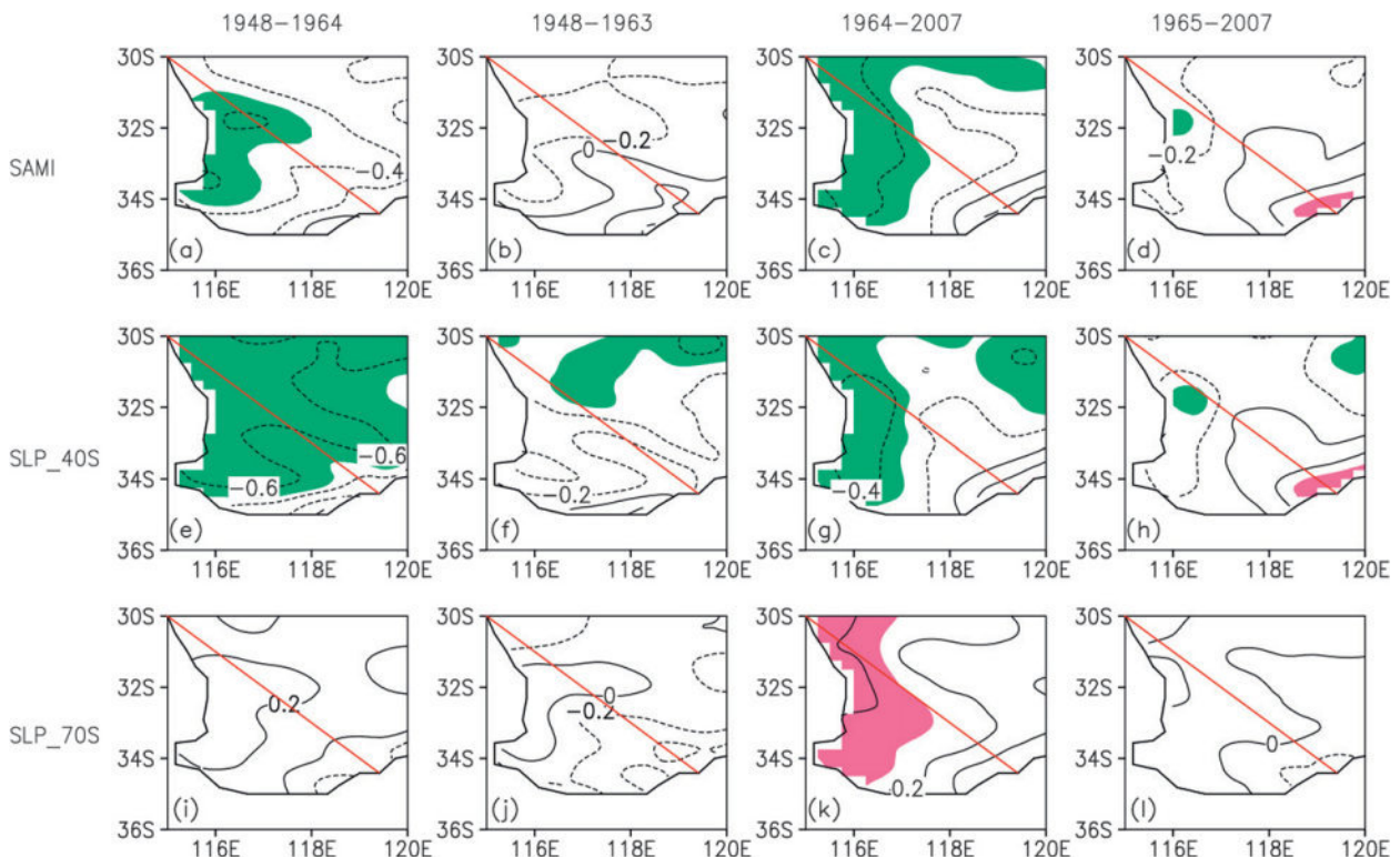
FIG. 3. Spatial distribution of the correlation coefficients between the winter SAMI and SWWA winter rainfall during (a) 1948–64, (b) 1948–63, (c) 1964–2007, and (d) 1965–2007. The second (e)–(h) and third (i)–(l) rows are the same as the first, but for the correlation between the SWR and zonal mean SLP at 40° and 70°S, respectively. Red (green) shading denotes regions of positive (negative) significance at the 0.05 level. The SWWA area lies southwest of the red line joining 115°E, 30°S and 120°E, 35°S.
