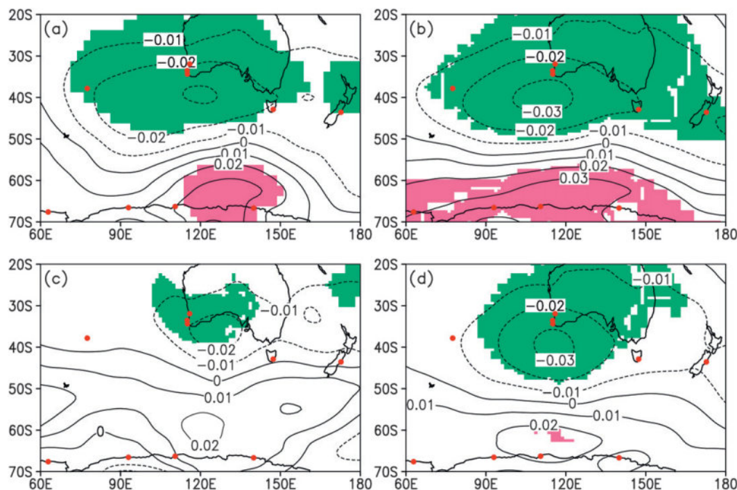
FIG. 4. Regression patterns of simultaneous SLP with respect to SWR for (a) 1948–64, (b) 1964–2007, (c) 1948–63, and (d) 1965–2007. Red (green) shading denotes regions of positive (negative) significance at the 0.05 level. Red dots indicate the locations of stations listed in Table 2.
