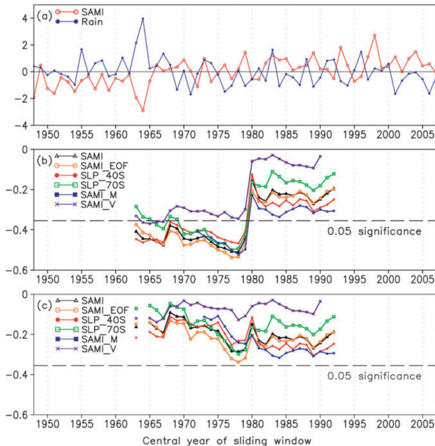
FIG. 1. (a) Normalized time series of the winter SAMI (red line) and SWWA winter rainfall (blue line). (b) Time series of detrended correlation coefficients using a 31-yr sliding window between SWR and each of winter SAMI (black line), SAMI_EOF (yellow line), zonal mean SLP at 40°S (red line), zonal mean SLP at 70°S (green line), SAMI_M (blue line), and SAMI_V (purple line). The sign of the relation between the zonal mean SLP at 70°S and SWR is reversed to enable a direct comparison with other data. (c) As in (b), but excluding the data for extreme year 1964.
